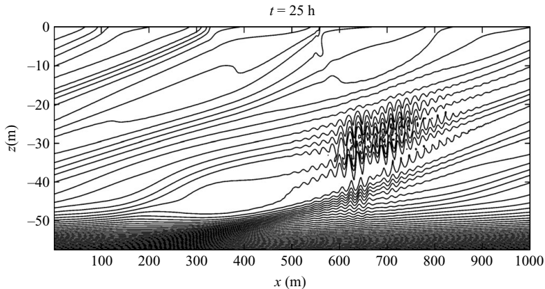
FIGURE 4. Isopycnals at a time just after the onset of the secondary K-H instability. Note that only a portion of the simulation domain is shown in order to focus on the small-scale features in the mixed layer.
