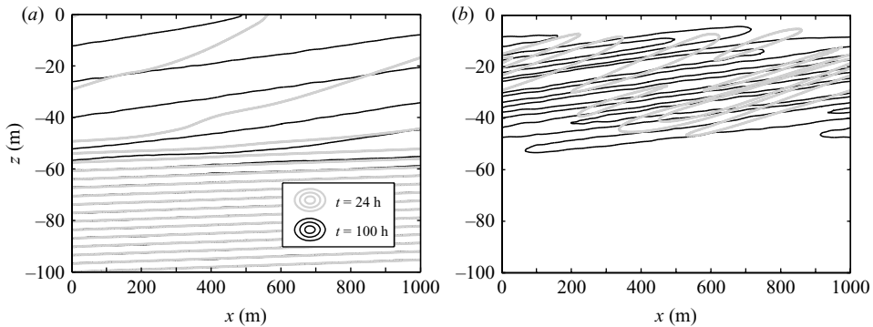
FIGURE 3. (a) Isopycnals and (b) velocity magnitude immediately preceding and following the period of active K-H instability, at t = 24 h (grey) and t = 100 h (black). The contour interval for isopycnals is 0.03 \text{ kg m}^{-3} and that for velocity magnitude is 0.01 \text{ m s}^{-1} .
