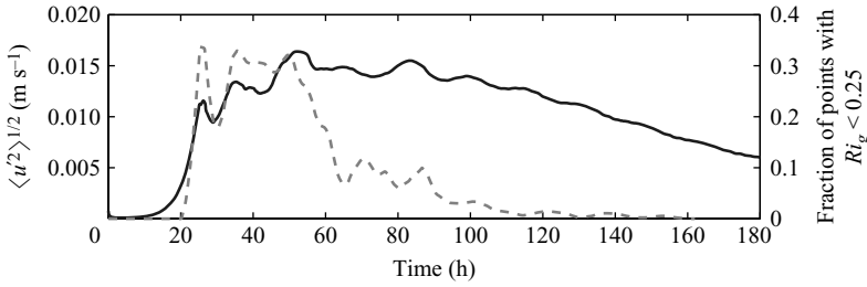
FIGURE 1. Temporal evolution of root mean square cross-front velocity (solid line) and the fraction of points with Ri_g < 0.25 (dashed curve), both averaged throughout the mixed layer, -50 \text{ m} < z < 0 .
