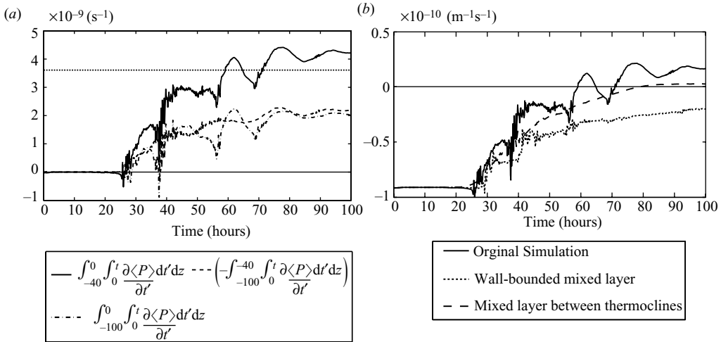
FIGURE 5. (a) Temporal change in the depth-integrated mixed-layer PV (solid line) with approximate fluxes from the thermocline (dashed line) and the upper surface (dash-dotted line). The increase in integrated PV needed to bring the entire mixed-layer PV to zero is indicated by a dotted line. (b) Volume-averaged mixed-layer PV for the three different simulations described in the legend. In order to remove the influence of the diffusive flux at the mixed layer/thermocline interface, the average excludes the 10 m bordering the thermoclines.
