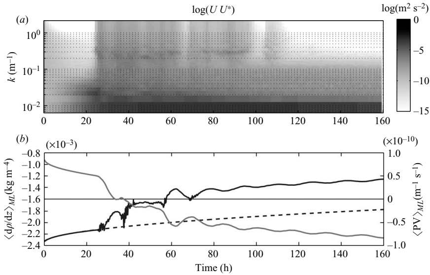
FIGURE 2. (a) Spectral energy of the streamwise velocity as a function of horizontal wavenumber and time, averaged over -50 < z < 0 ; (b) temporal evolution of Ertel's PV (grey) and the density gradient (black) averaged throughout the mixed layer. The dashed line shows the diffusive solution.
