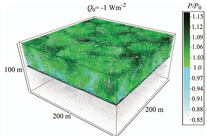
Fig. 6. Visualization of the phytoplankton concentration from the large-eddy simulation with a surface heat flux of Q_0 = -1 W m ^{-2} . The density surface bounding the base of the mixed layer is shown in gray and instantaneous streamlines are shown in white.
