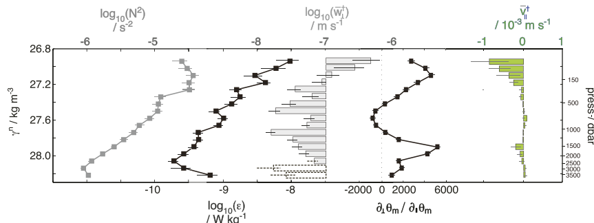
FIG. 9. Section-characteristic profiles of \log_{10}(N^2) , \log_{10}(\epsilon) , \log_{10}(\bar{w}_{\perp}^t) , \partial_{\perp}\theta_m/\partial_{\parallel}\theta_m , and the contribution to \bar{v}_{\perp}^t balanced by dianeutral advection of mean potential temperature. Negative values of \bar{w}_{\perp}^t are indicated by dashed bars. The section-mean pressure profile of isoneutral surfaces is indicated on the right-hand axis.
