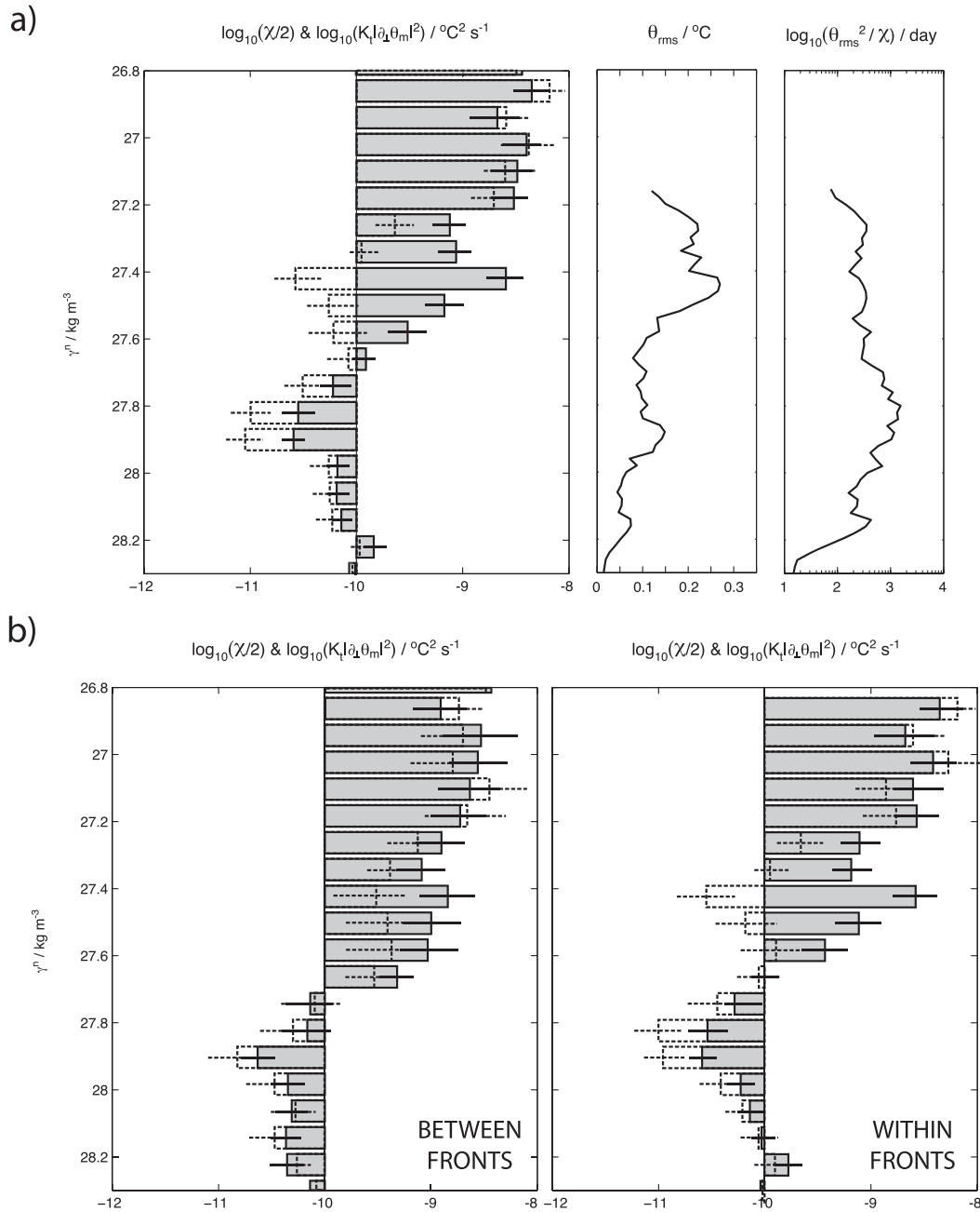
FIG. 5. (a) Mean profiles of (left) the rate of dissipation of temperature variance \chi/2 (gray bars) and the rate of dianeutral production of temperature variance K_l |\partial_{\perp} \theta_m|^2 (dashed bars), with uncertainties, for the JC69 occupation of the SR1b transect; (center) the rms potential temperature fluctuation in (10), estimated from all available SR1b hydrographic section repeats; and (right) the time scale of temperature variance dissipation, estimated as \theta_{\text{rms}}^2 / \chi using the data in the left and center panels. (b) As in (a), but partitioned into stations (left) between frontal jets and (right) within frontal jets; a station is defined to be within a frontal jet if the LADCP-measured speed exceeds 0.15 \text{ m s}^{-1} somewhere in the water column.
